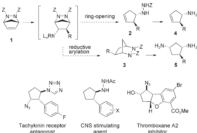
Scheme 1. Desymmetrization of strained alkenes by two competing pathways involving an initial enantioselective carbometalation. Z = electron withdrawing group.
